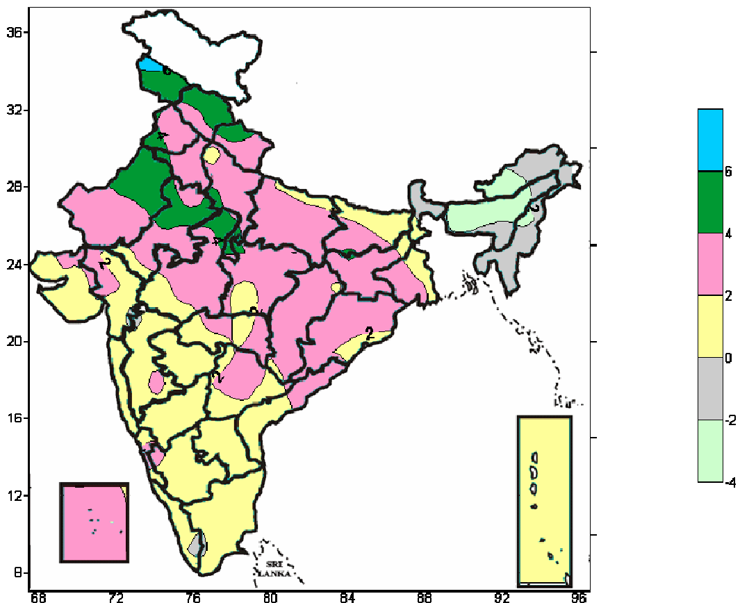
Maximum Temperature ( ^{\circ}\text{C} ) Anomaly in India for the week ending 07.02.07
