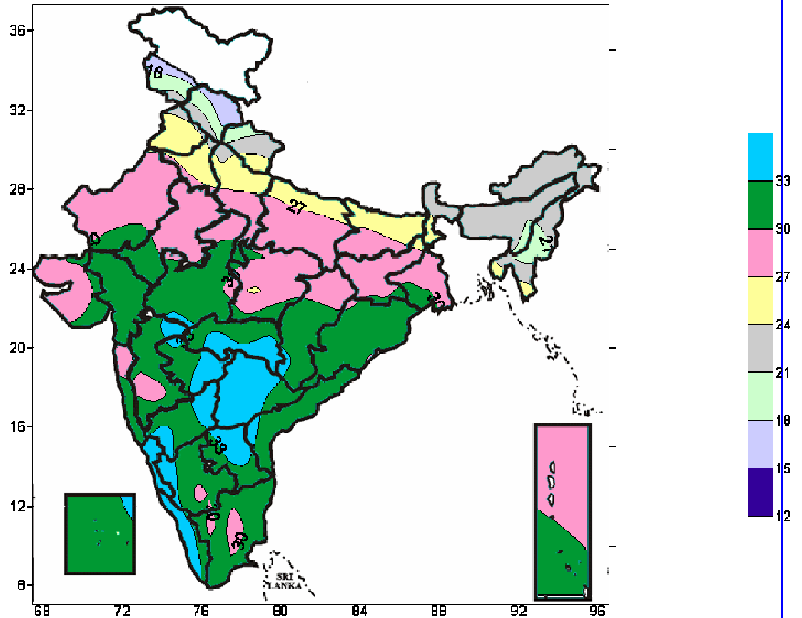
Actual mean maximum Temperature ( ^{\circ}\text{C} ) in India for the week ending 07.02.07
