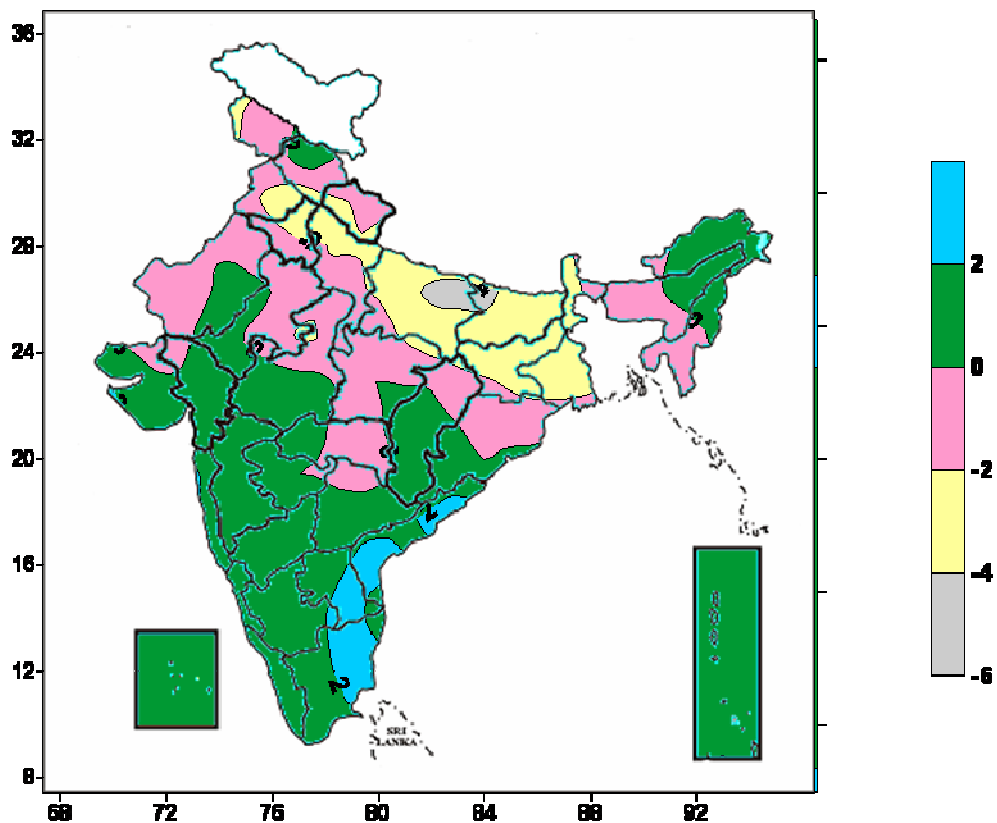
Maximum Temperature ( ^{\circ}\text{C} ) Anomaly In India for the week ending 21.03.07
