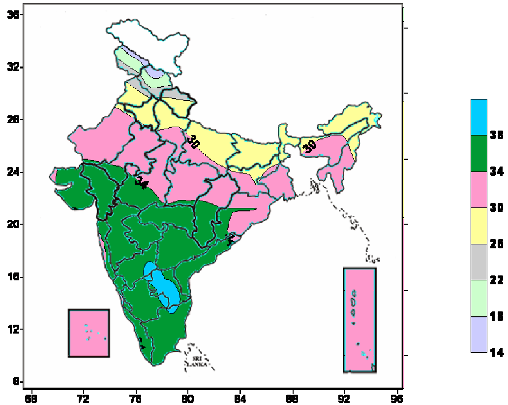
Actual mean maximum Temperature ( ^{\circ}\text{C} ) In India for the week ending 21.03.07
